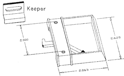
K-3077 Mill Finish K-3077B Brown K-3077W White
