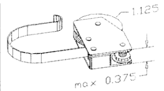
90021 WHEEL PLASTIC 90021A WHEEL METAL CLOSED-END (MALE)
