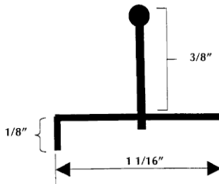
PSDT-BOTTOM Clear Anodized Aluminum 6' or 12'
