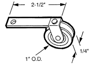
02506-1 Nylon Wheel 02506-5 Metal Wheel
