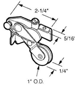
90036 Nylon Wheel 90036S Steel Wheel
