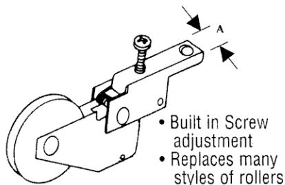
02518 A = 7/16" 02519 A = 5/16"
