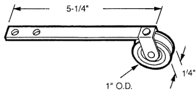
B-527 Nylon Wheel B-528 Steel Wheel
