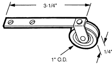
B-523 Nylon Wheel B-524 Steel Wheel
