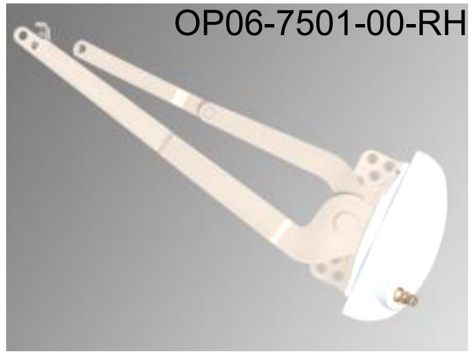
Right Hand X Drive CRS Dual Arm Operator with Vinyl Base
